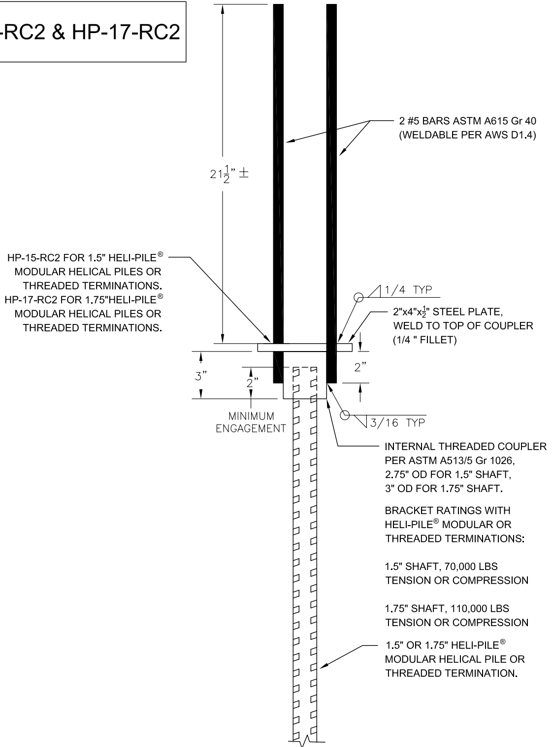
NEW CONSTRUCTION COMPRESSION BRACKET, HP-15-RC2 & HP-17-RC2 NO SCALE
